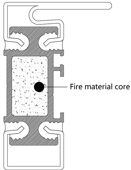
Fire steel profile
