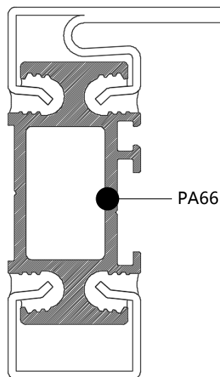
Steel thermally broken profiles
